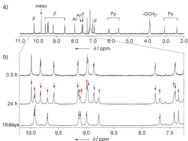
Figure 2. a) ^1\text{H} NMR spectrum ( \delta = 2.0 – 11.0 ppm) of [\text{ZnP}(\equiv)_2]_4 at 20^\circ\text{C} in [\text{D}_6]\text{benzene} , and b) its time-dependent change ( \delta = 7.2 – 10.2 ppm) after a change in the solvent to \text{CCl}_4 .
