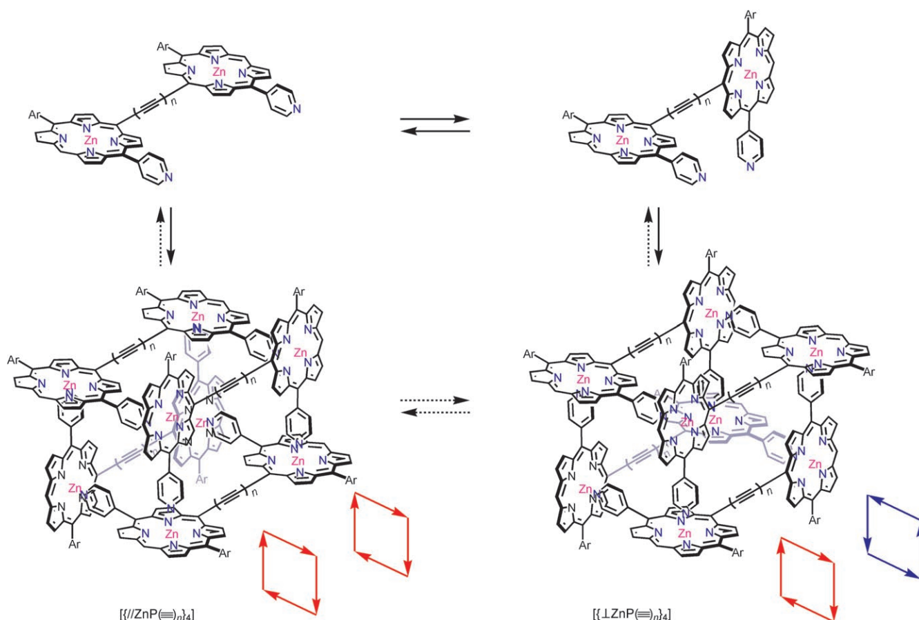
Scheme 1. Oligoalkynylene-bridged zinc bisporphyrin complexes [ZnP(\equiv)_n] ( n = 1, 2, \text{ and } 4 ) and their cyclic tetramers. Red and blue arrows indicate the directions of the dipole moments.
